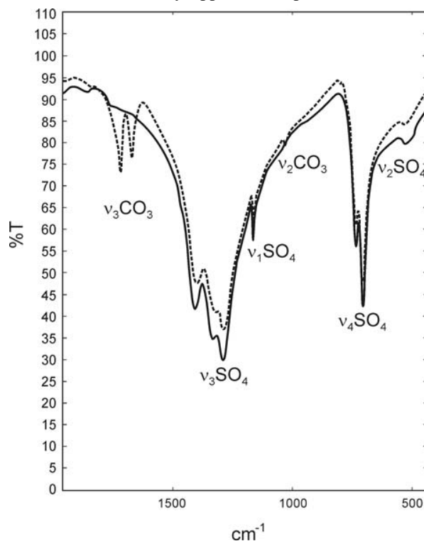
Fig. 2. IR spectra of endogene (bold line) and supergene (dashed line) barite from the Kremikovtsi deposit.
