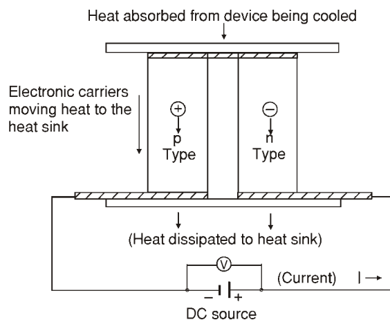
Figure 10. Thermoelectric architecture for cooling electronic equipment
