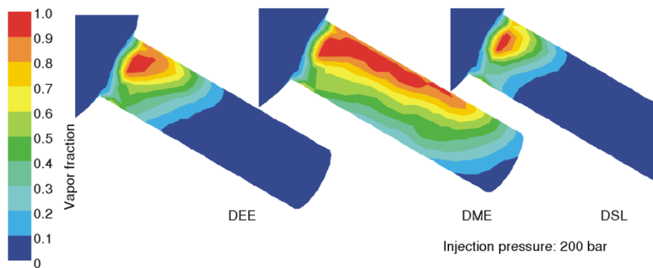
Figure 3. Vapor fraction at injection pressure of 200 bar (color image see on our web site)
