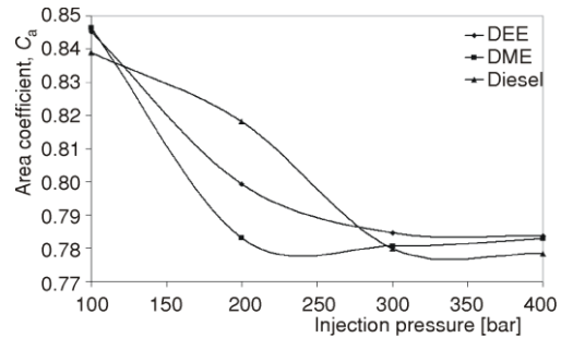
Figure 9. Variation of the area coefficient with injection pressure
