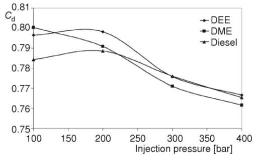
Figure 8. Variation of the discharge coefficient with injection pressure
