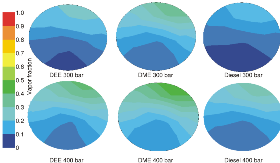
Figure 4. Vapor fraction at the nozzle outlet for injection pressures of 300 bar and 400 bar (color image see on our web site)
