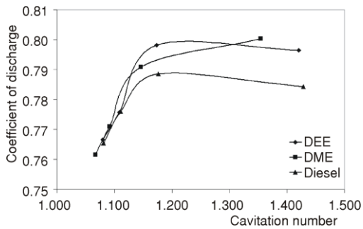
Figure 10. Variation of the discharge coefficient with cavitation number
