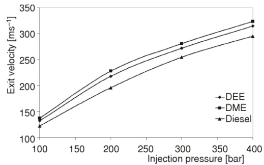
Figure 11. Variation of the exit velocity with injection pressure
