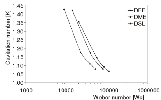
Figure 7. Variation of cavitation number with Weber number
