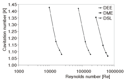
Figure 6. Variation of cavitation number with Reynolds number
