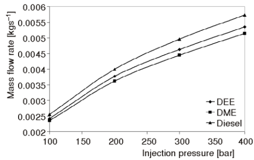
Figure 12. Variation of the mass flow rate with injection pressure
