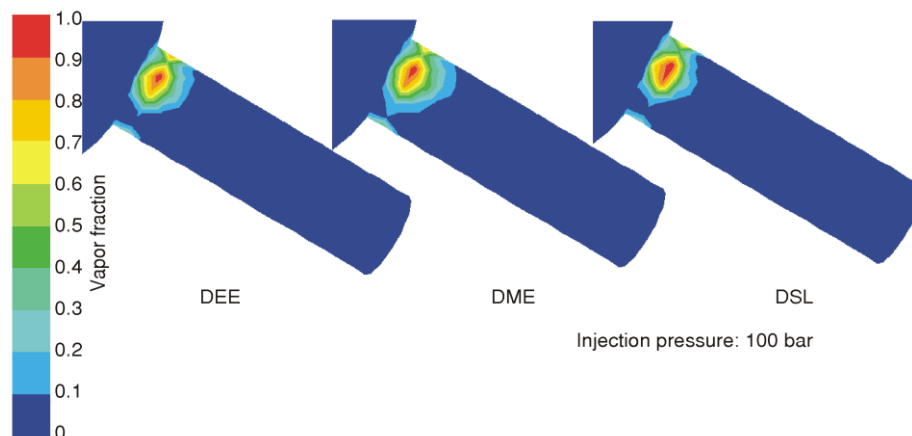
Figure 2. Vapor fraction at injection pressure of 100 bar (color image see on our web site)
