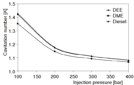
Figure 5. Variation of cavitation number with injection pressures
