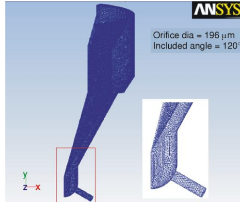
Figure 1. Mesh generated for the 120° sector of the injector (color image see our on web site)
