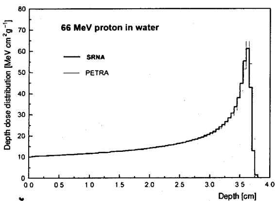
Figure 5. Monte Carlo simulation of depth dose distribution in water for 66 MeV protons beam
