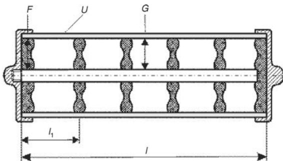
Figure 2. Five segment GM counting chamber
