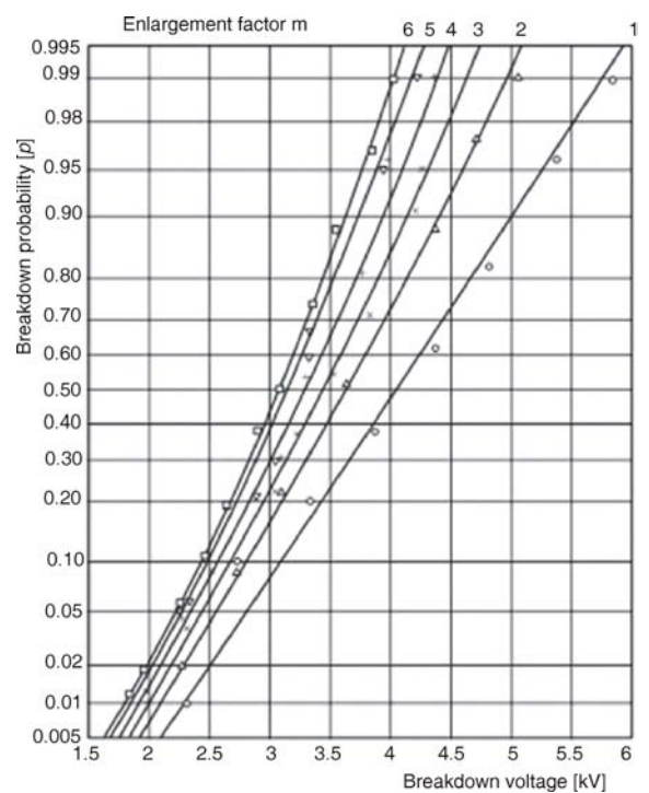
Figure 7. Validity of the enlargement law for the m segment GM model
