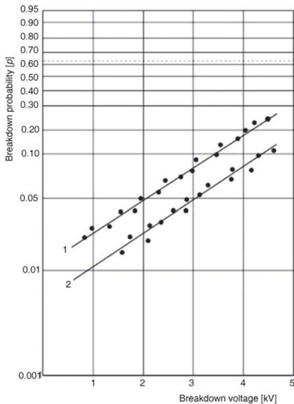
Figure 6. Surface breakdown voltage over spacer, displayed on probability paper of the double-exponential distribution; 1 – type I spacer; 2 – type II spacer
