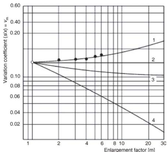
Figure 8. Random variable variation coefficient as a function of enlargement factor m (number of segments) and the appropriate theoretical dependencies for: 1 – double-exponential distribution, 2 – two parameter Weibull distribution, 3 – normal distribution, 4 – three parameter Weibull distribution
