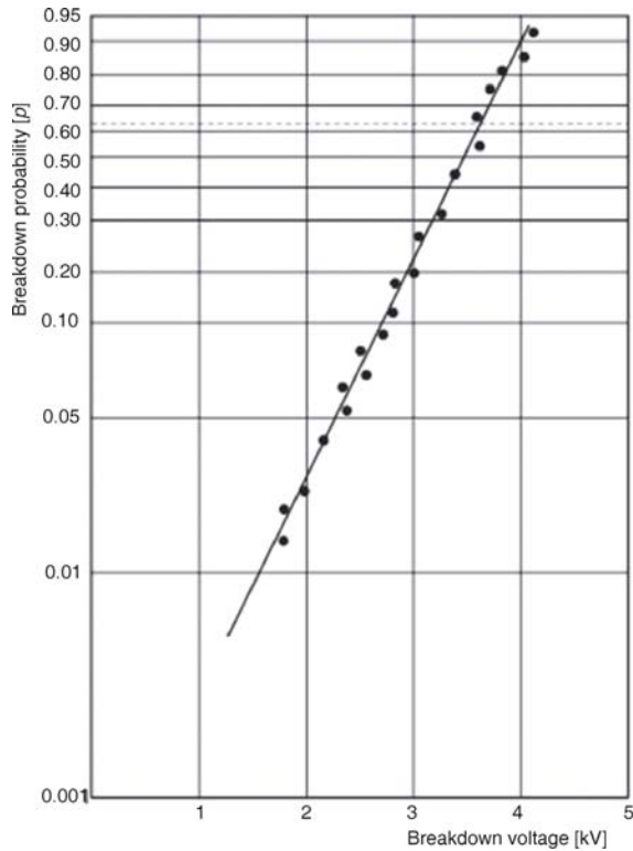
Figure 5(b). Breakdown voltage of the GM counter model (fig. 1) with type II spacer, displayed on probability paper of the double-exponential distribution
