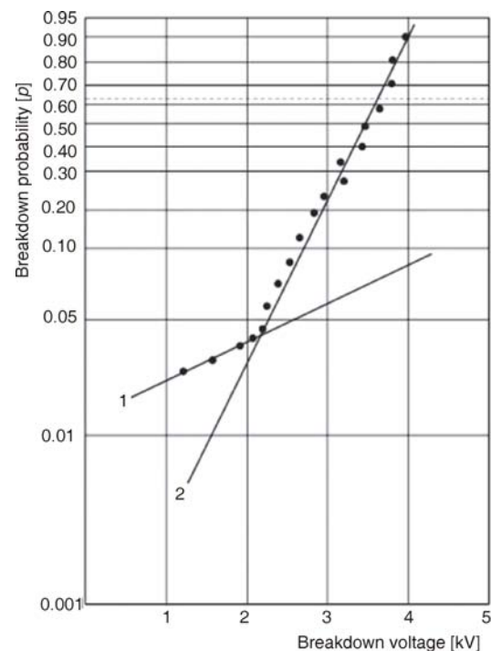
Figure 5(a). Breakdown voltage of the GM counter model (fig. 1) with type I spacer, displayed on probability paper of the double-exponential distribution
