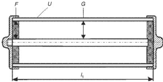
Figure 1. Segment of a GM counter chamber
