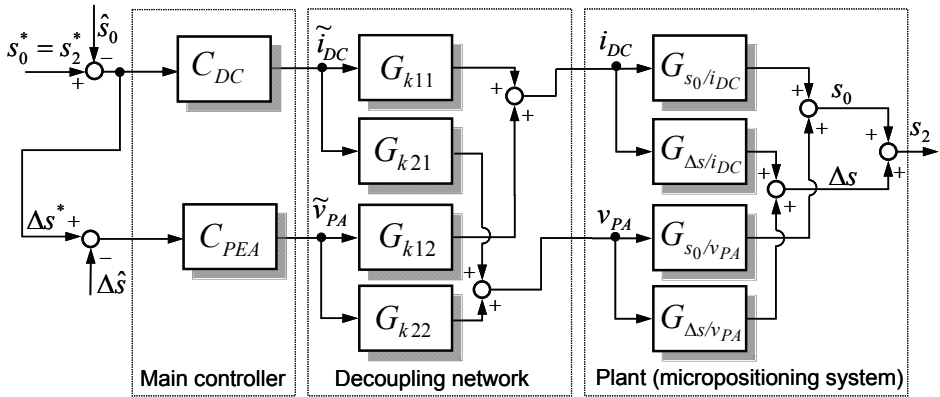
Fig. 4 – The integrated control structure.
