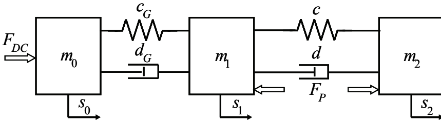
Fig. 5 – Simplified plant model of the micropositioning stage.
