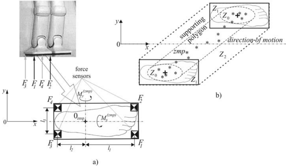
Fig. 3 – Zero-Moment Point.
