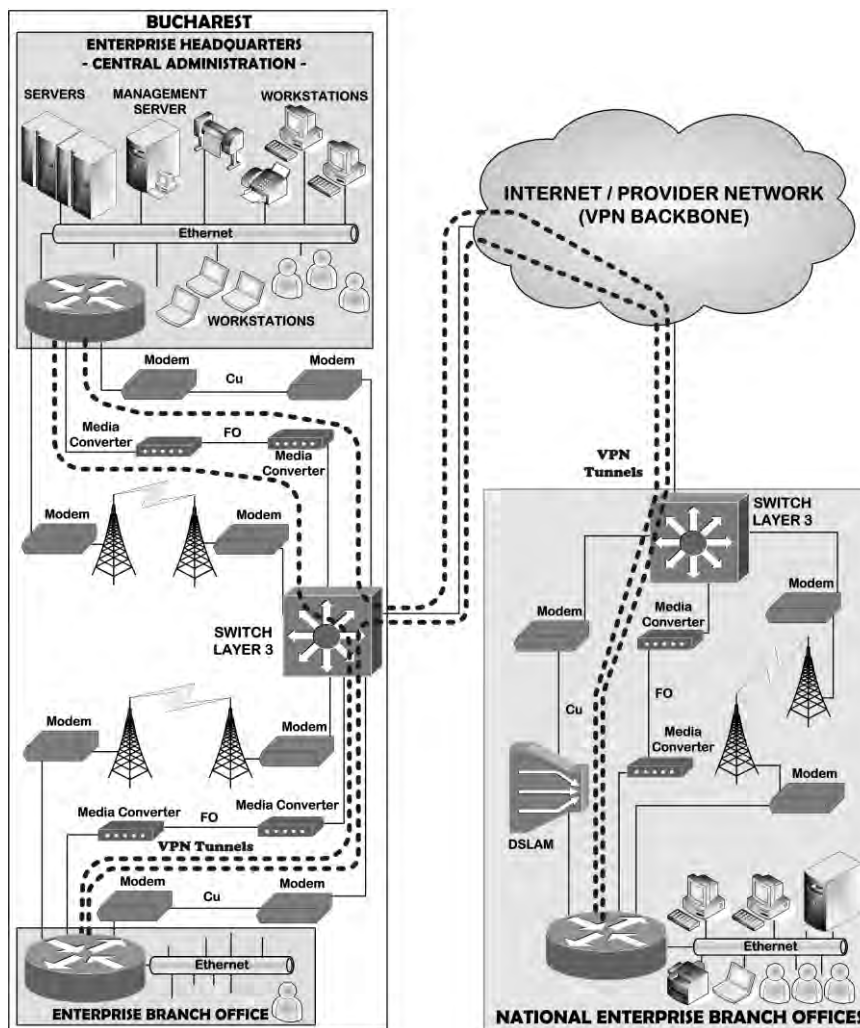
Fig. 11. A network general architecture with 3 loops (copper, fiber optic and radio), using the Internet or a provider network, for a large enterprise geographically dispersed to support transfer of large volumes of data over long distances
