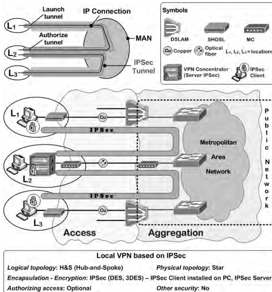
Fig. 13. Local VPN based on IPsec example
