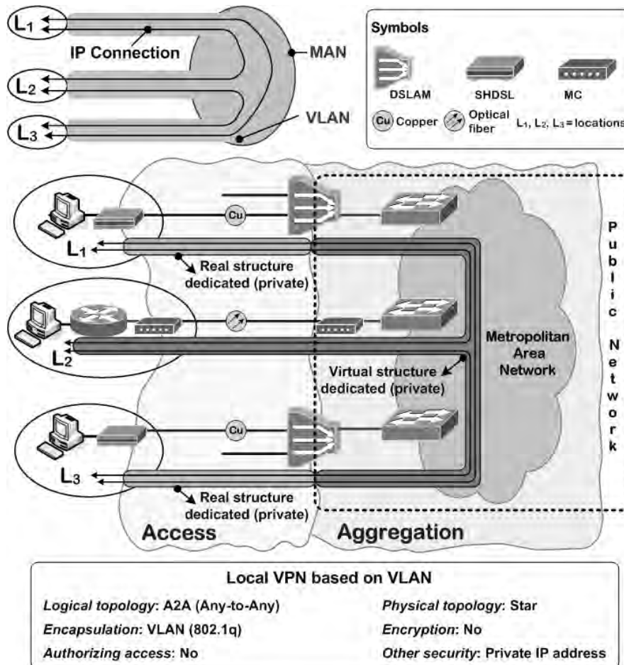
Fig. 12. Local VPN based on VLAN example
