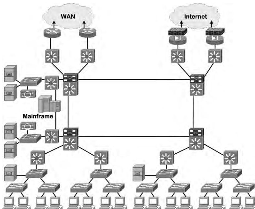
Fig. 10. A hierarchical scalable network design model
